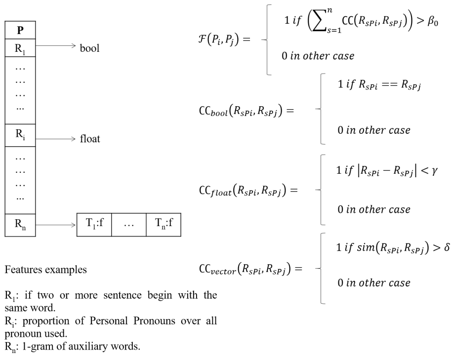
Figure 1. Description of paragraph representation and similarity function
