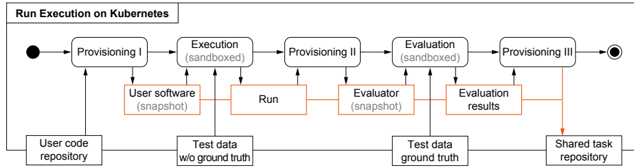
Figure 1. UML activity diagram of the control flow (rounded boxes) and the data flow (rectangular boxes). All run artifacts (highlighted middle “row”) are persisted through the provisioning steps in the shared task repository. The user software and evaluator are “untrusted” software and therefore run in a sandbox without network access.
